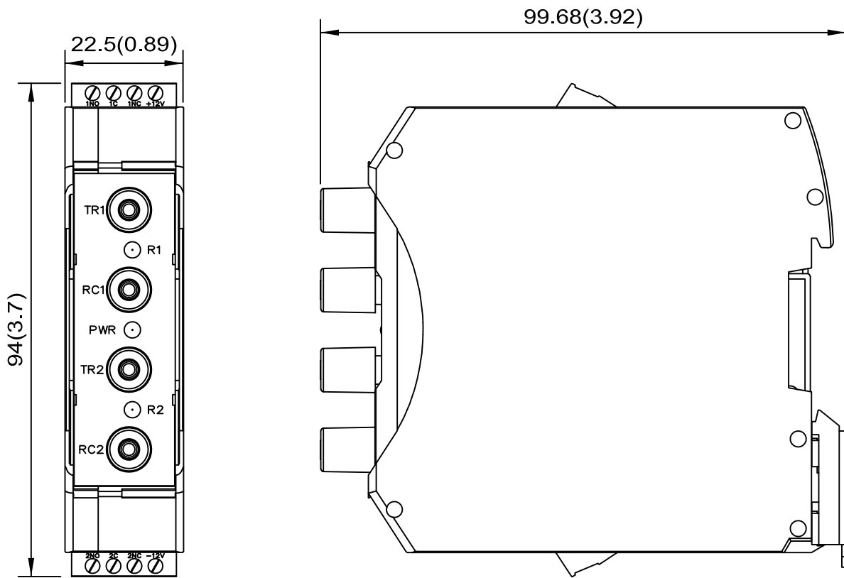
Transceiver
